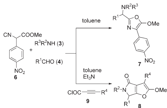
Scheme 2. Multicomponent synthesis of 5-methoxyoxazoles 7 and furopyrrrolones 8 .
