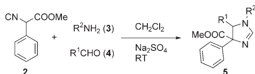
Scheme 1. Three-component synthesis of imidazolines described by Orru and co-workers.
